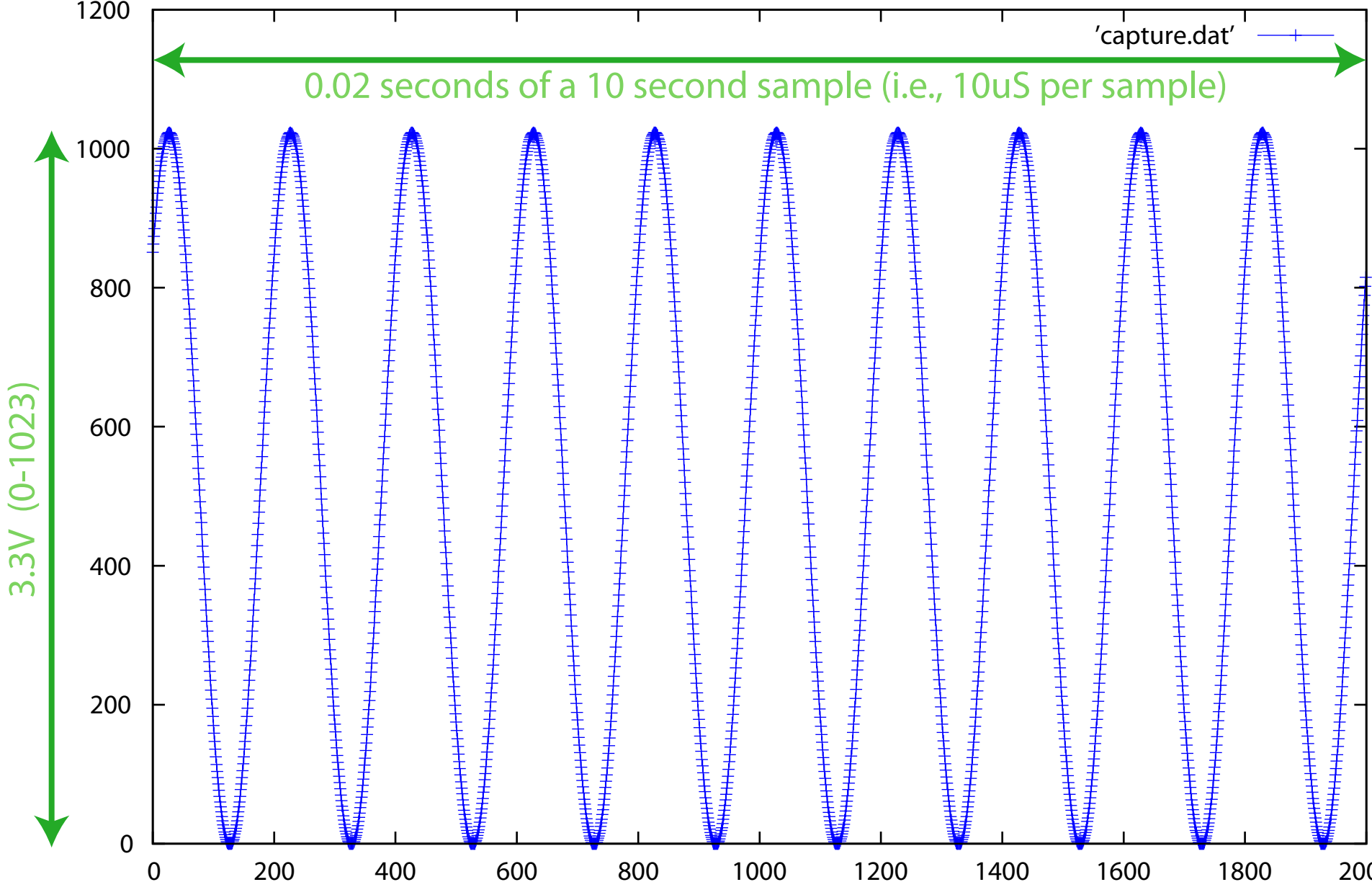
EBB ADC Example: First 2,000 of 1,000,000 samples @ 100KSps
